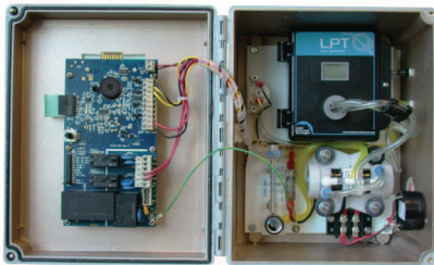
Inside of the DCC-SD showing an LPT-A gas detector with a toxic, combustible or refrigerant sensor on right hand side of the enclosure.
